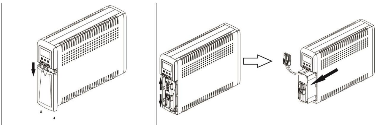
Figure 4 - Battery Replacement
